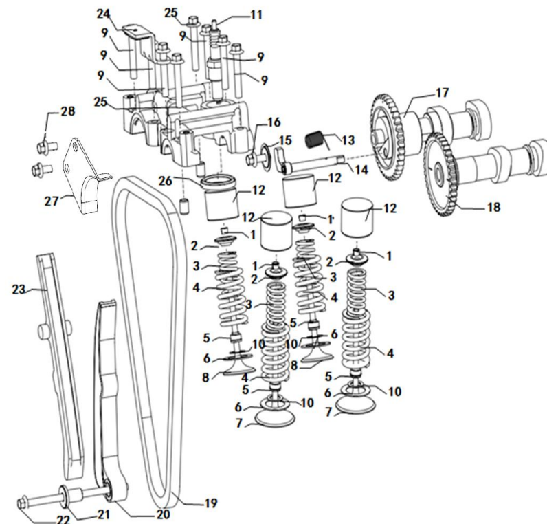
配气机构 VALVE MECHANISM
